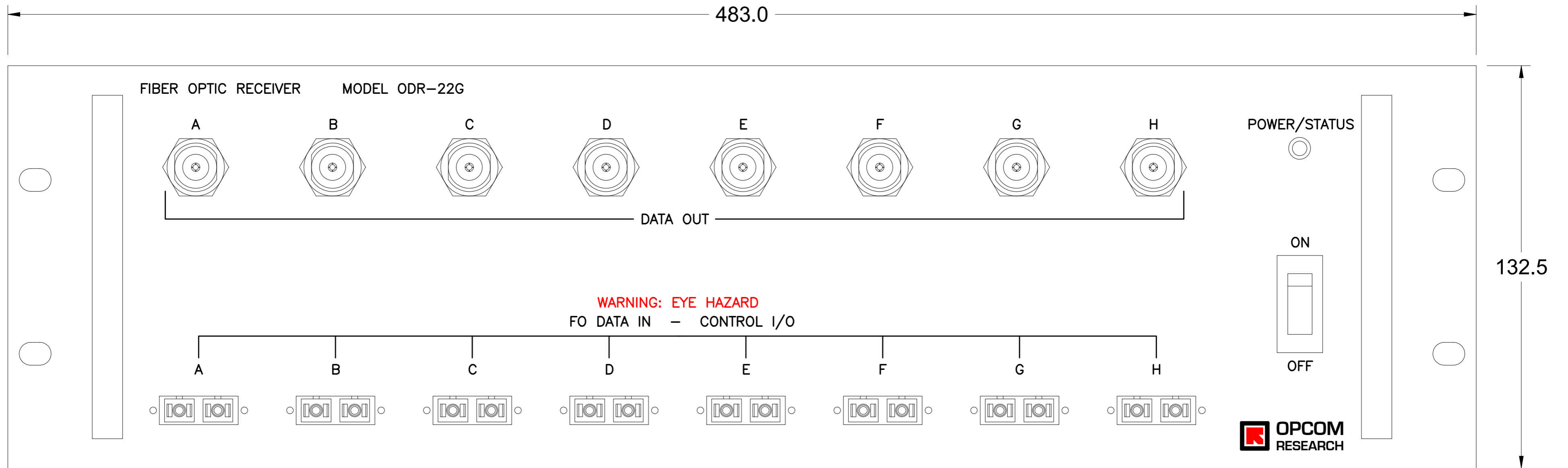
ODR-22G Front Panel (19 in rack mount version)
