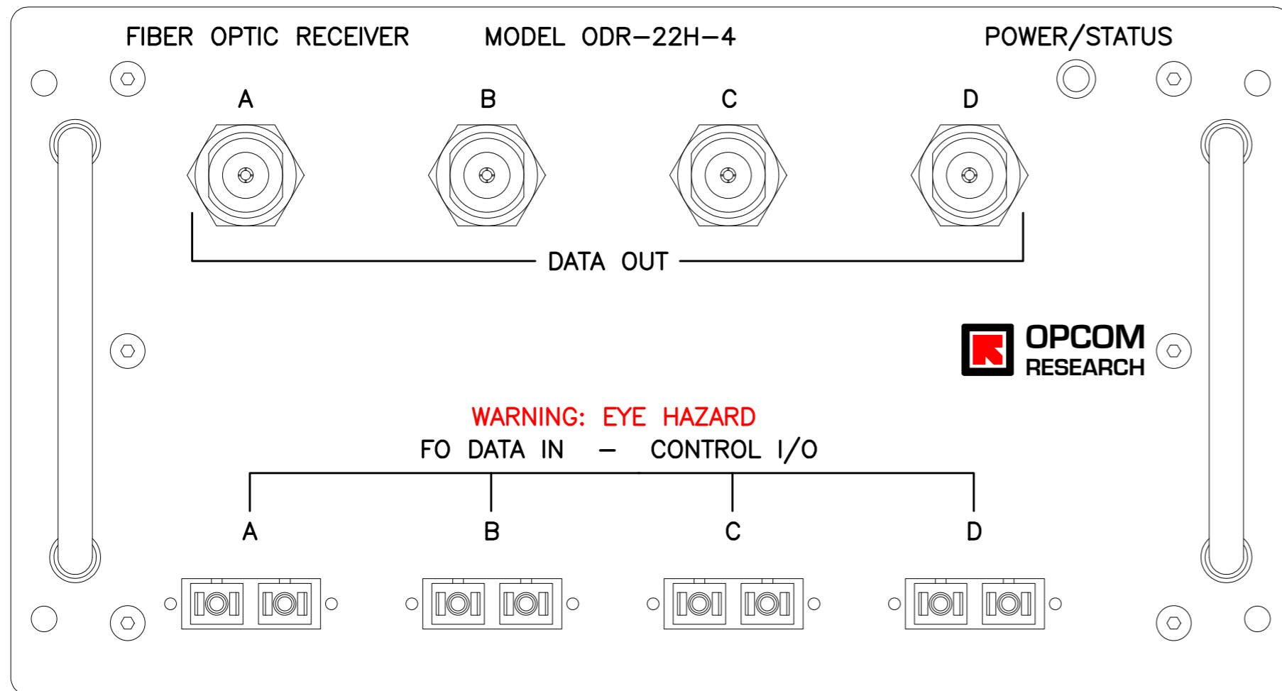
ODR-22H-4 Front Panel (desktop version)
