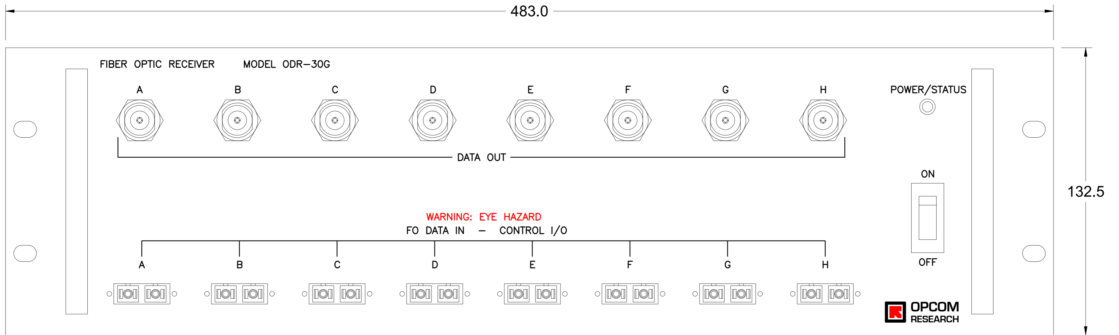
ODR-30G Receiver Front Panel (19 in rack mount version)
