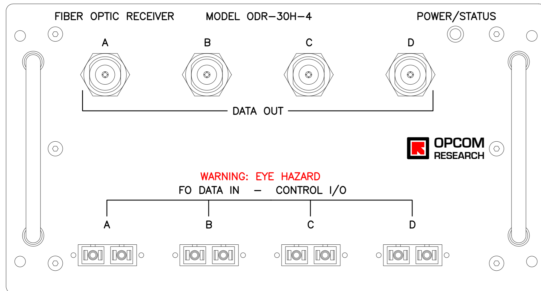
ODR-30H-4 Receiver Front Panel (desktop version)
